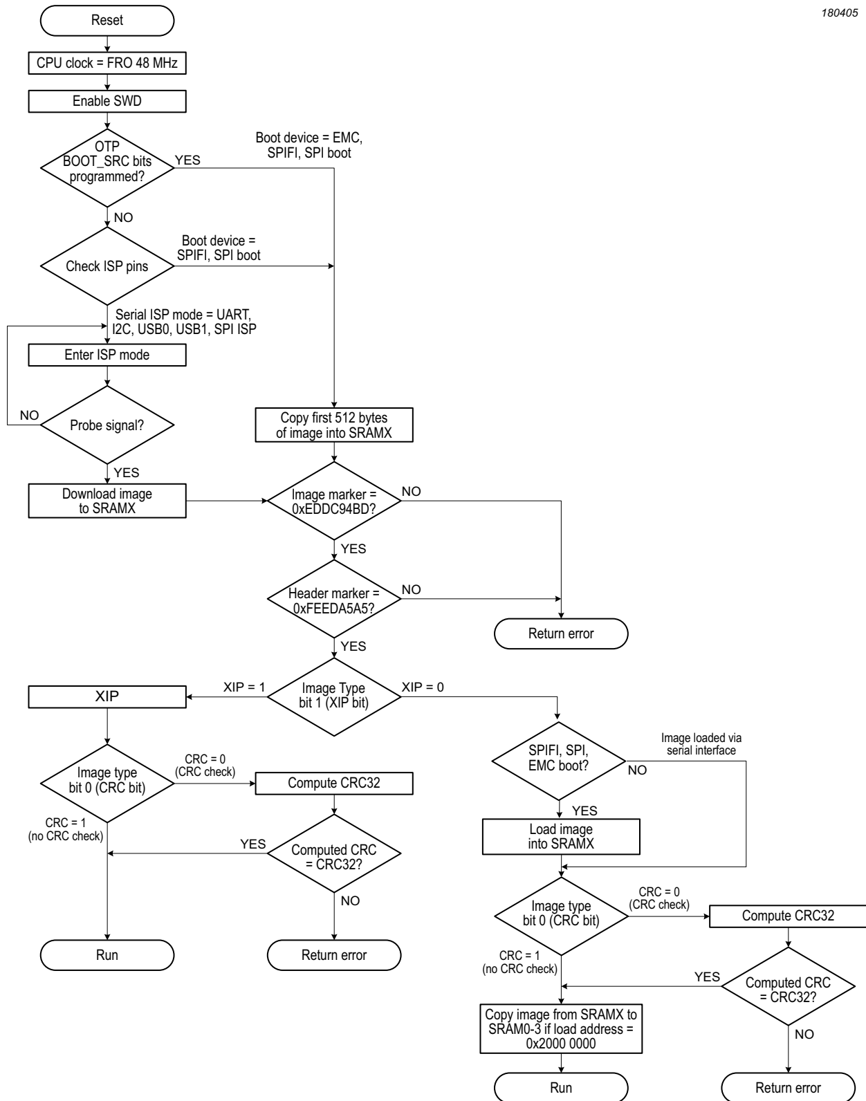
Fig 4. LPC54018JxM boot process flow chart
