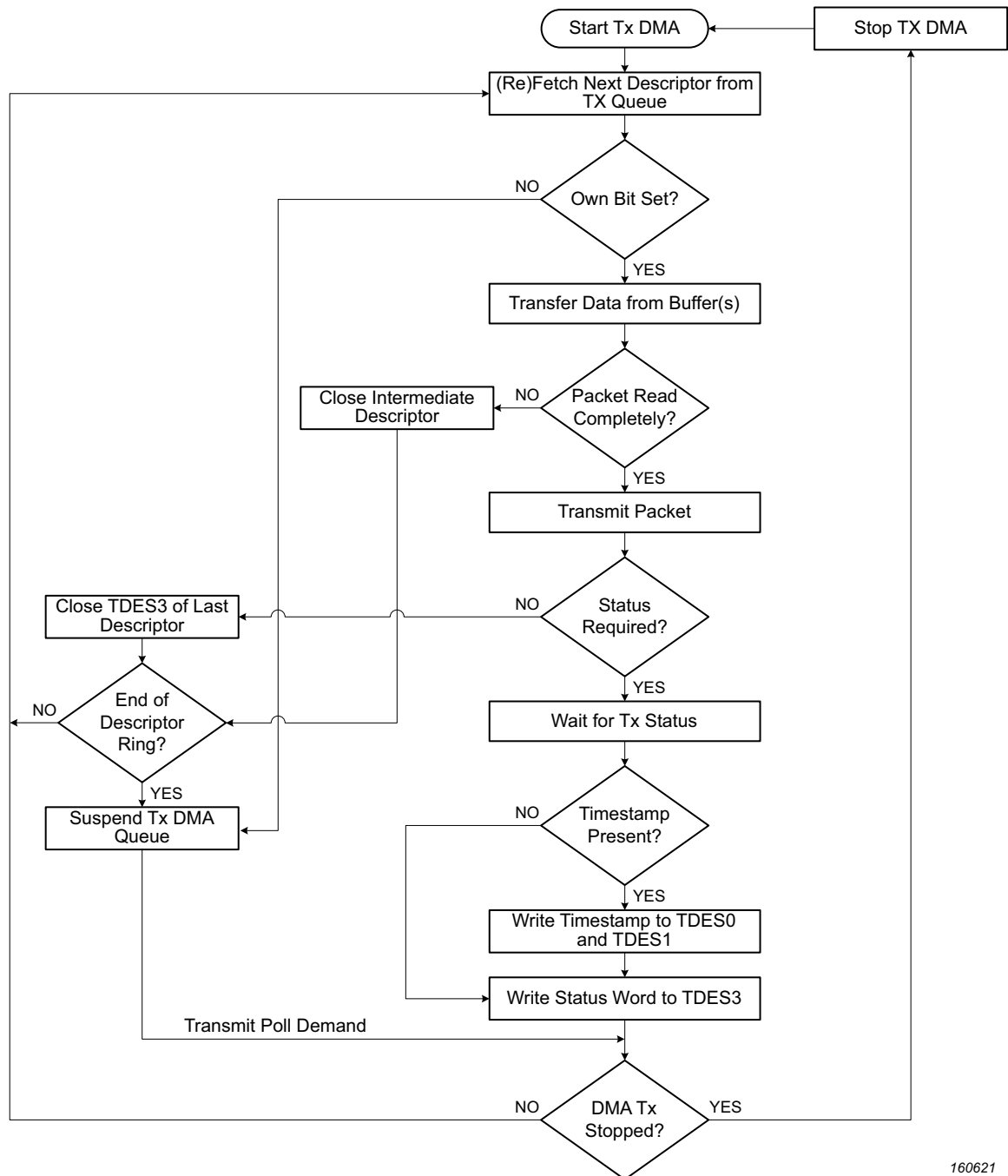
Fig 162. Transmit DMA operation in default mode
