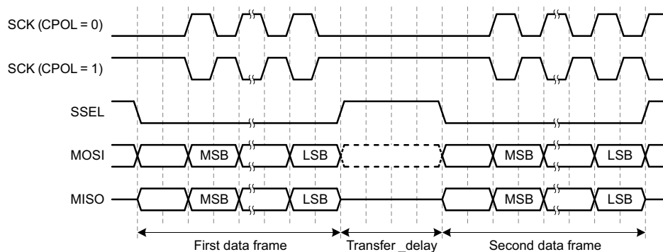
Fig 74. Transfer_delay
