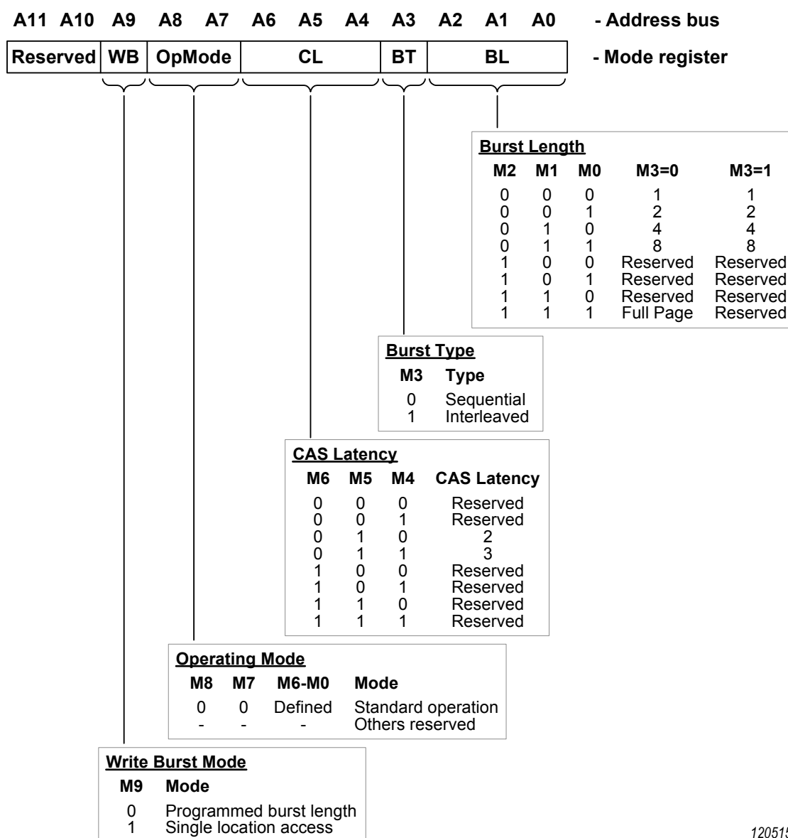
Fig 125. SDRAM mode register
