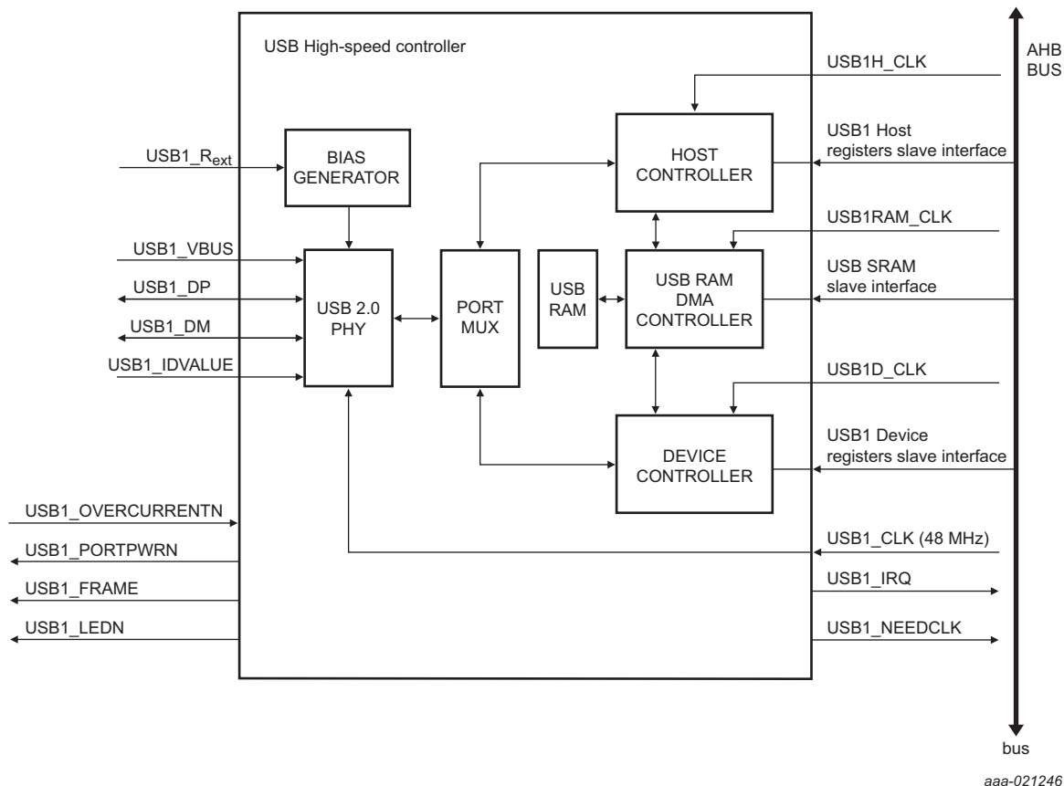
Fig 179. USB Host/Device controller block diagram
