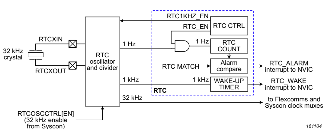
Fig 62. RTC clocking and block diagram
