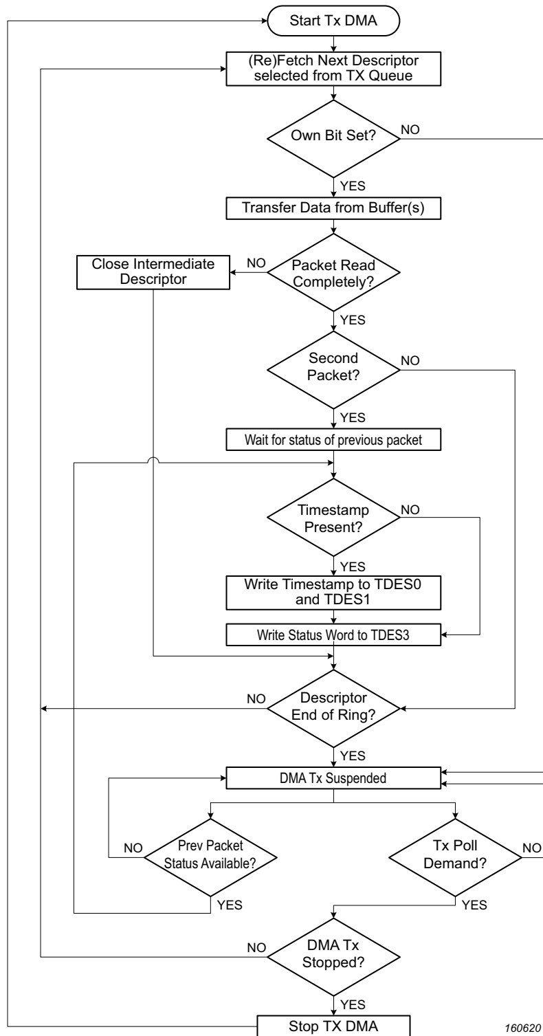
Fig 163. Transmit DMA operation in OSF mode
