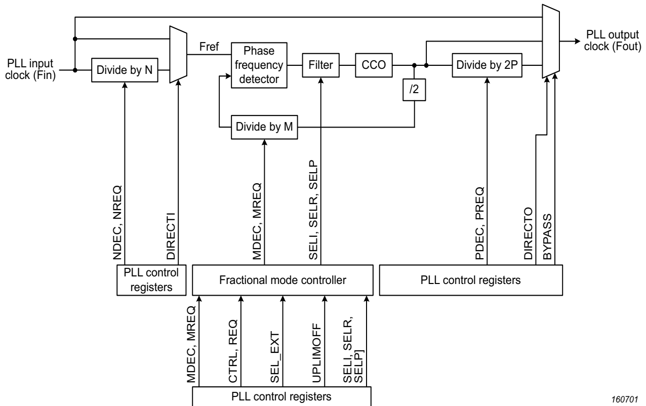
Fig 27. Audio PLL block diagram showing typical operation
