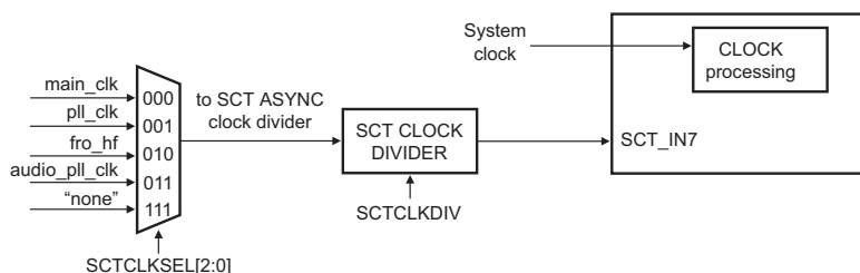
Fig 41. SCTimer/PWM clocking
