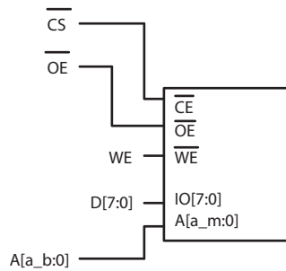
Fig 128. 8 bit bank external memory interface (bits MW = 00)
