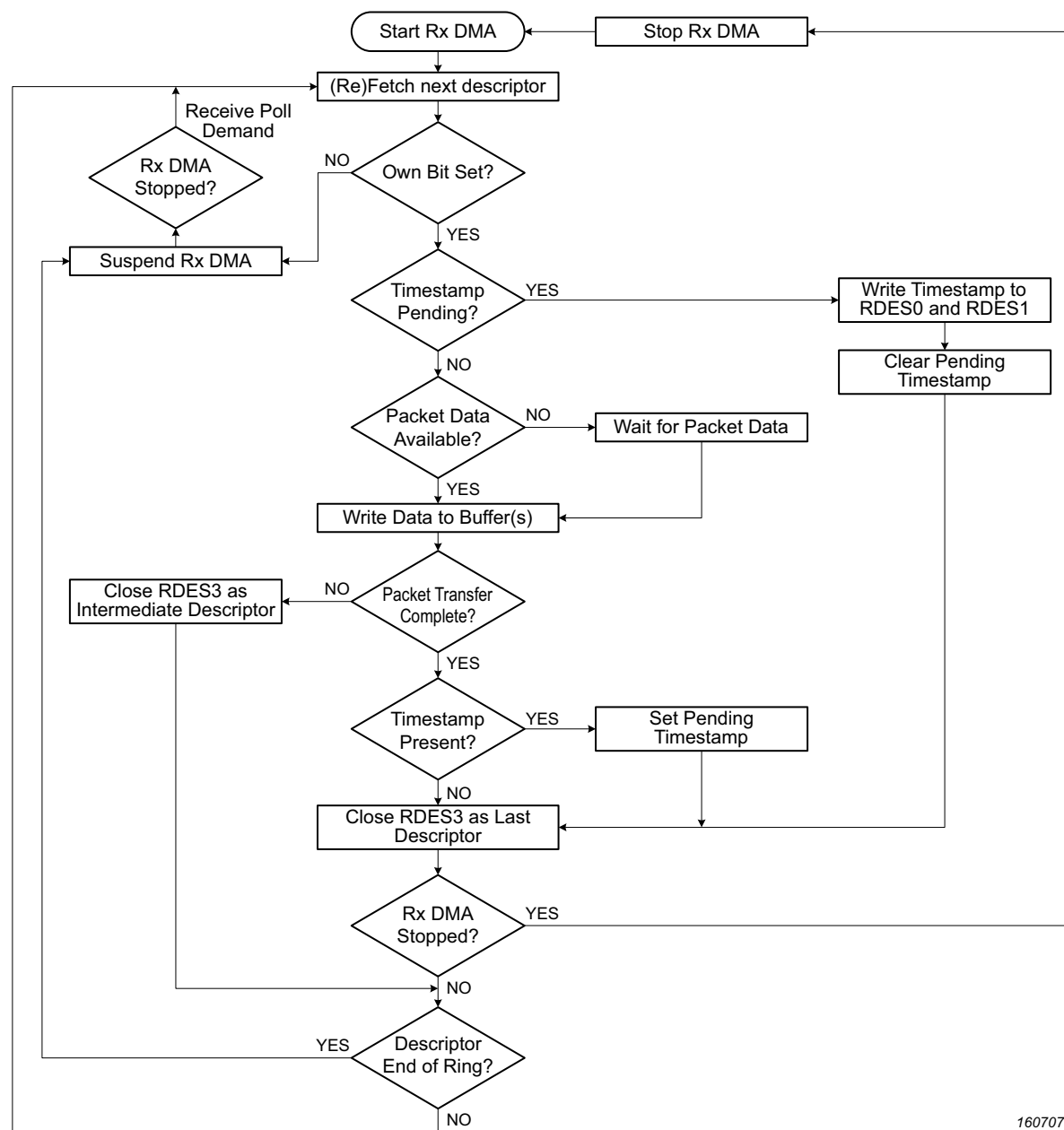
Fig 165. Receive DMA operation
