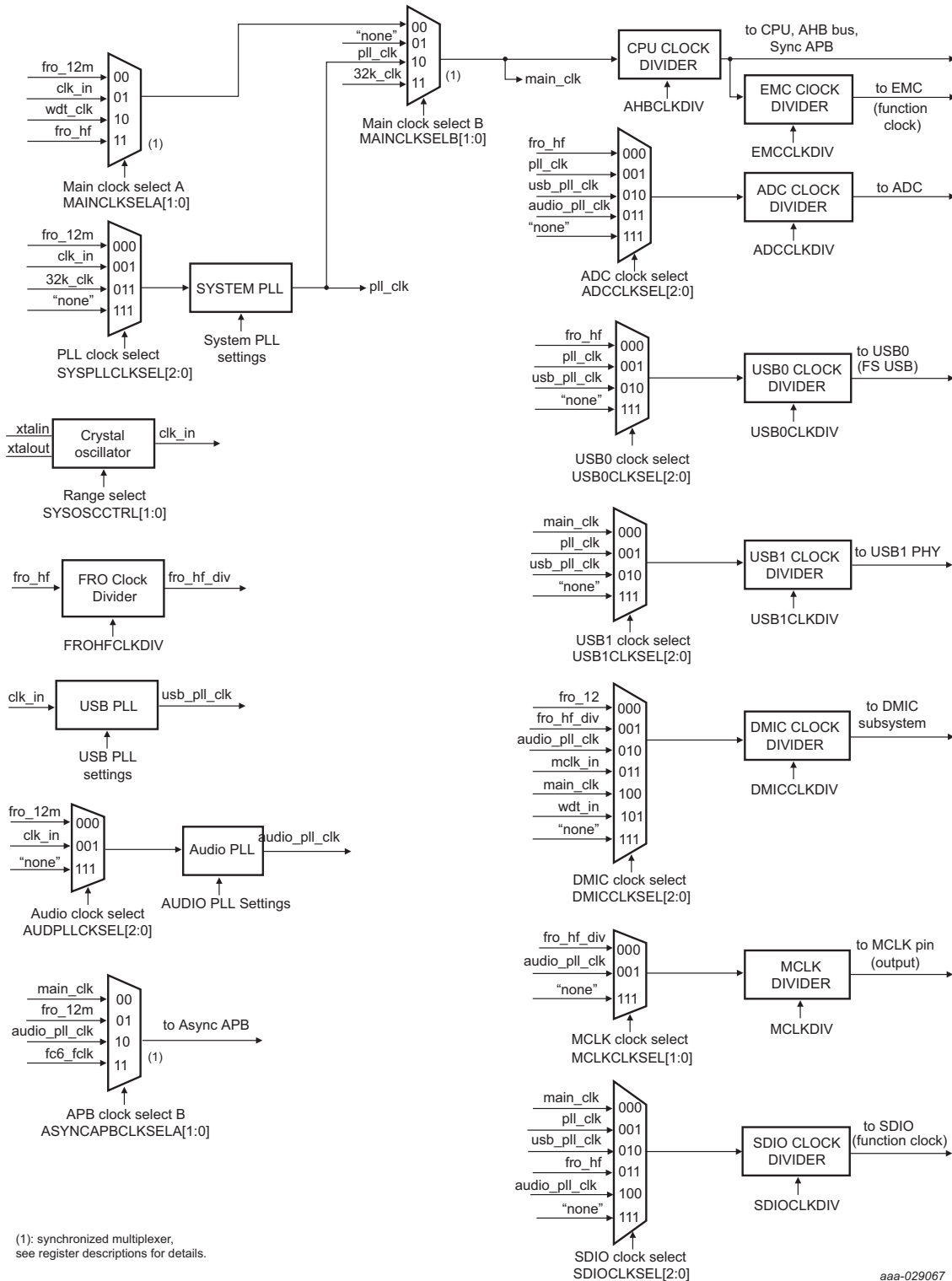
Fig 21. Clock generation
