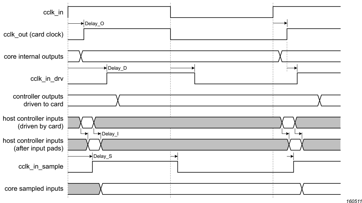
Fig 119. Clock relationship
