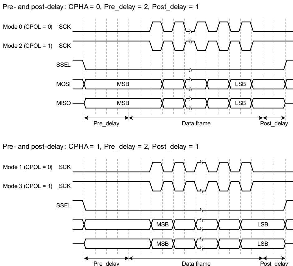
Fig 72. Pre_delay and Post_delay
