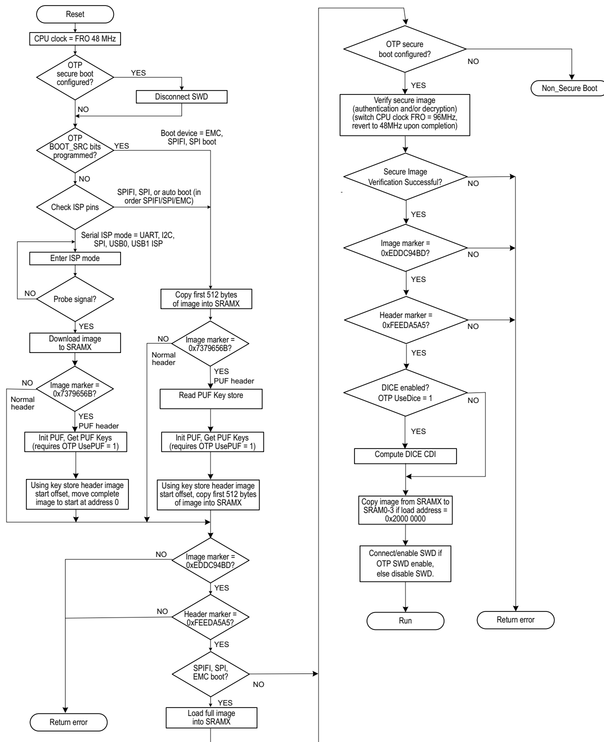
Fig 6. LPC54S018JxM boot process flow chart
