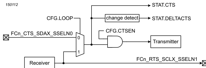
Fig 69. Hardware flow control using RTS and CTS
