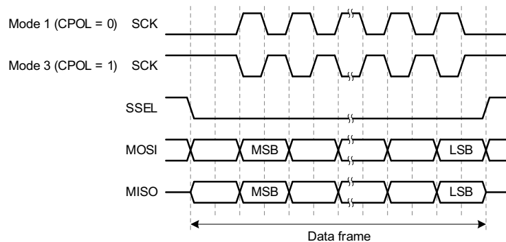
Fig 71. Basic SPI operating modes
