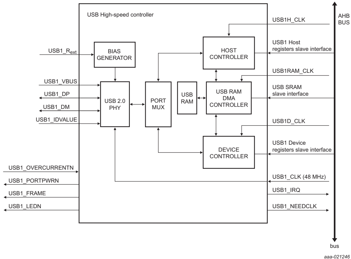
Fig 184. USB Host controller block diagram
