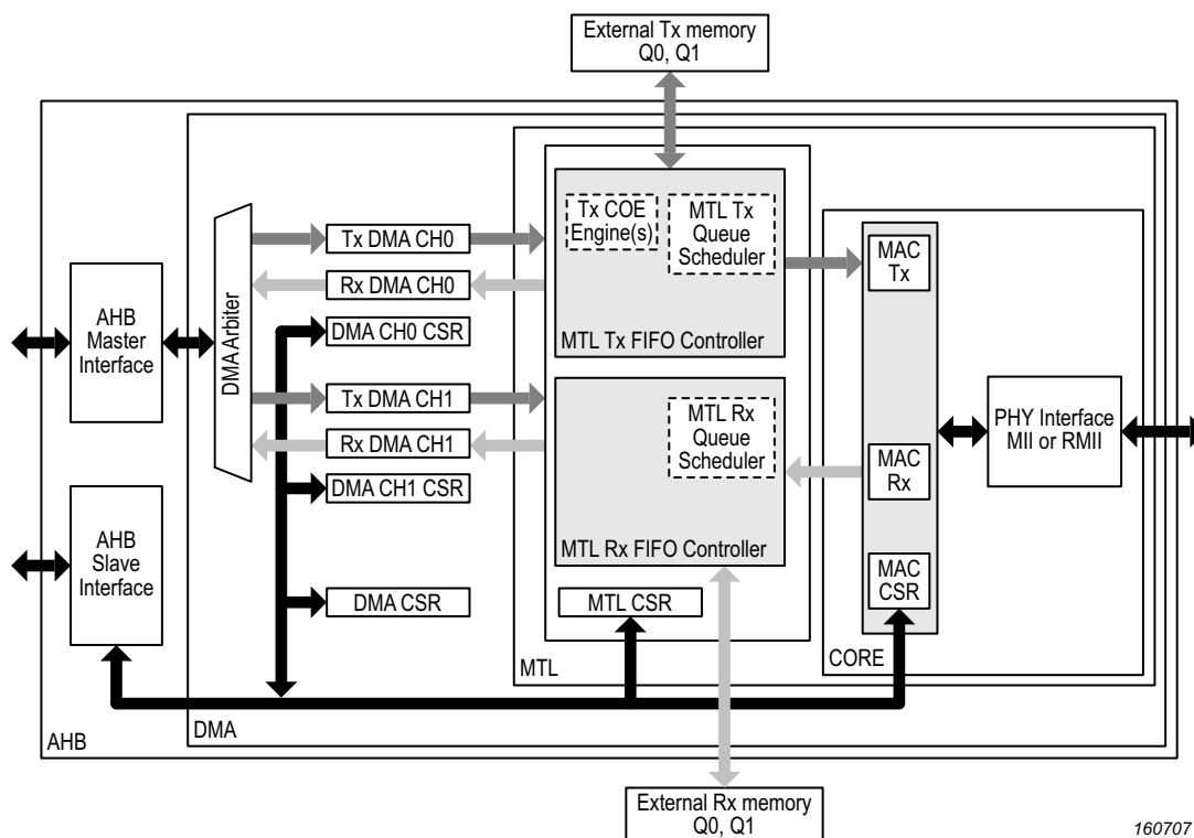
Fig 157. Multiple channels and queues
