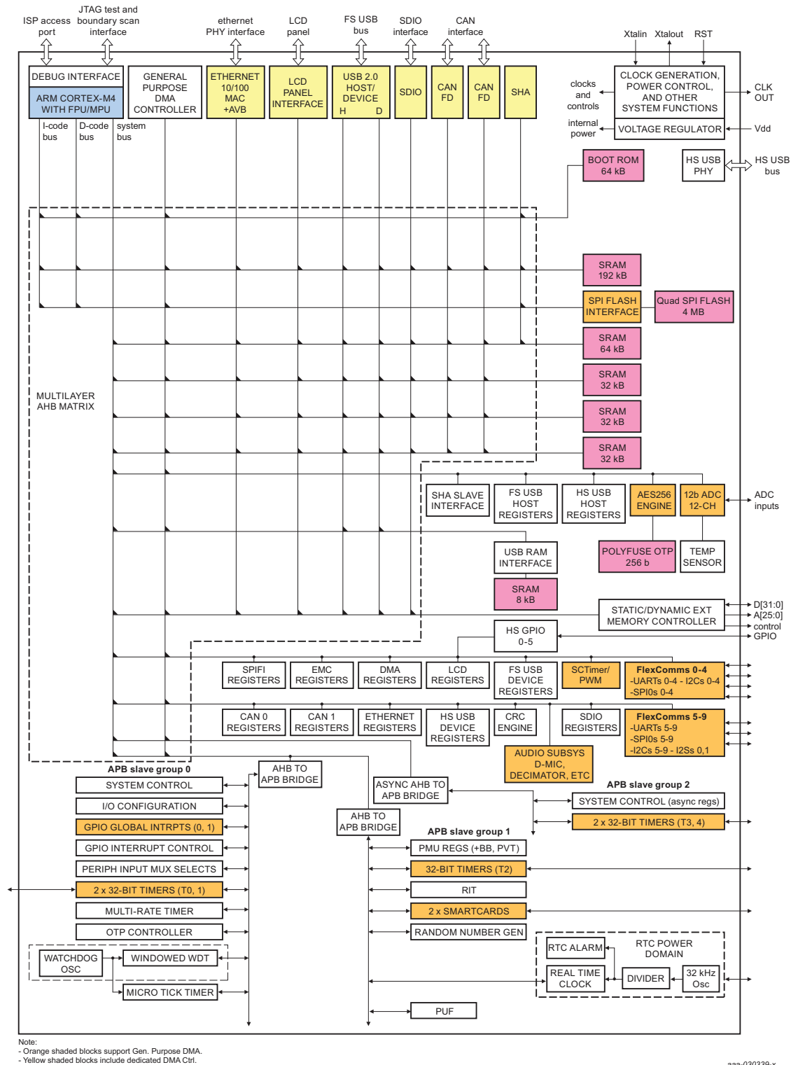
Fig 1. Block diagram
