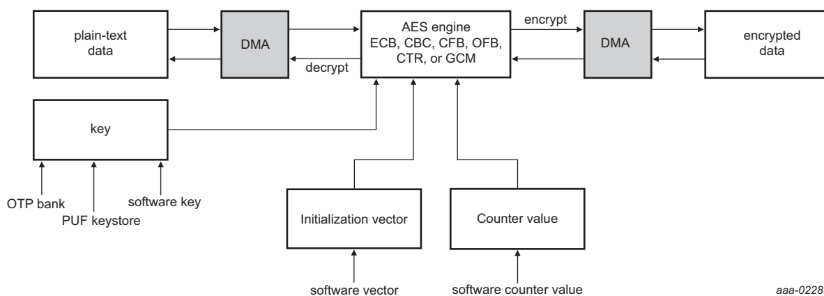
Fig 195. AES data encryption/decryption
