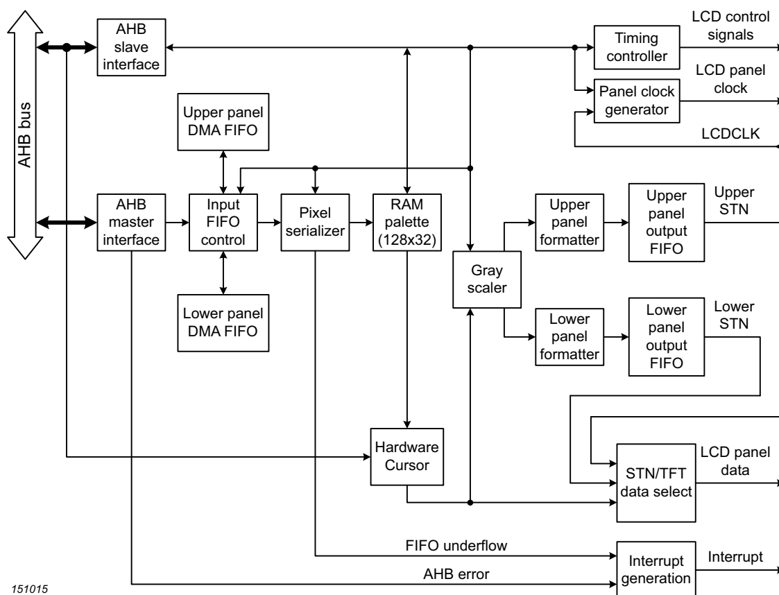
Fig 130. LCD controller block diagram
