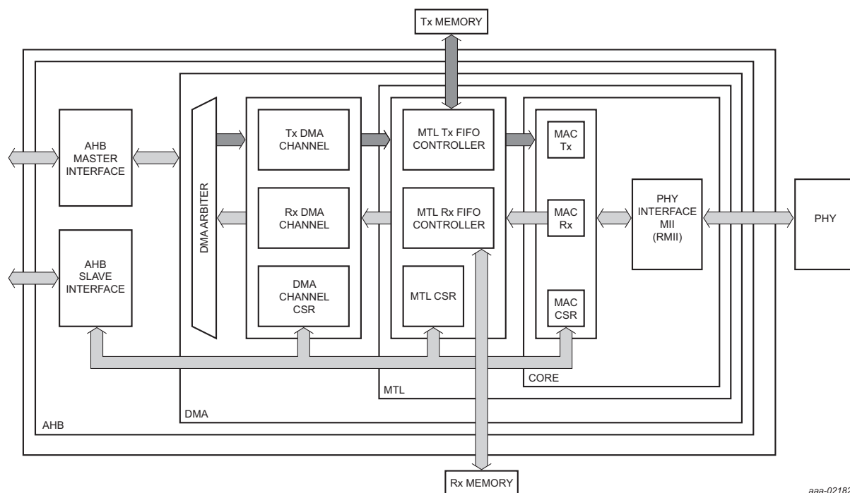
Fig 155. Ethernet block diagram
