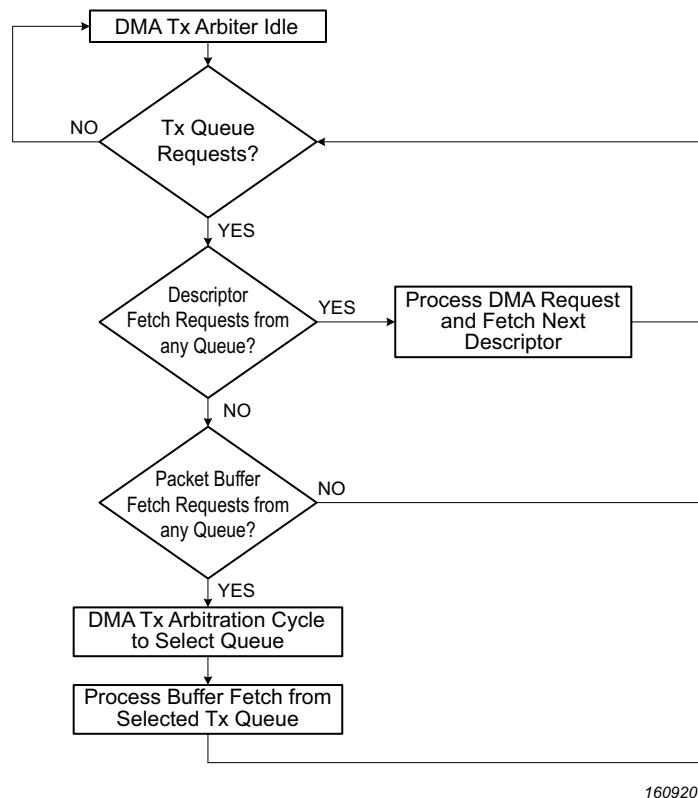
Fig 164. DMA transmit channel arbitration process
